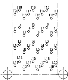
CONNECTOR PIN-OUT DETAIL COMPONENT SIDE OF BOARD DETAIL F SCALE: 2:1
